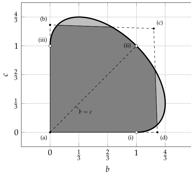
Fig. 3. A plot of the set of positive but not completely positive maps \Phi_{b,c} . The gray region indicates the values of (b, c) for which \Phi_{b,c} is positive. For every point (b, c) in the gray region, with the exception of the dashed line b = c , the map \Phi_{b,c} is indecomposable, and hence is able to detect entanglement in some PPT state. The curved part of the boundary (i.e., the thick black line) consists of exposed positive maps. The four points (a)–(d) are the points described by Theorem 3, and hence every map in the dark gray region is incapable of detecting entanglement in absolutely PPT states. The point (i) is the Choi map \Phi_C , (iii) is its dual \Phi_C^\dagger , and (ii) is the reduction map. This figure is also reproduced and considered in the following works [49, 48]
