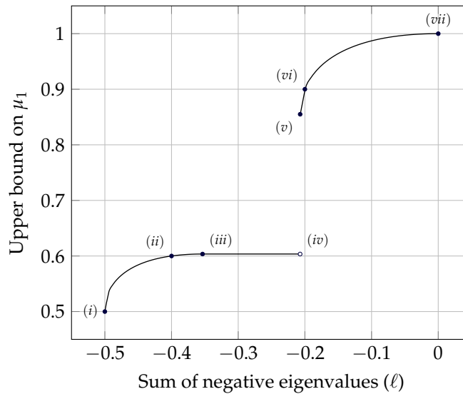
Fig. 2. A plot of the upper bound f(\ell) given by Lemma 2. For example, point (i) is (-\frac{1}{2}, \frac{1}{2}) , which tells us that if the sum of the negative eigenvalues ( \ell ) of W equals -\frac{1}{2} then W cannot detect entanglement in absolutely PPT states if the largest eigenvalue ( \mu_1 ) of W is \leq \frac{1}{2} . Point (ii) corresponds to \ell = -\frac{2}{5} and \mu_1 \leq \frac{3}{5} , (iii) corresponds to \ell = -\frac{1}{2\sqrt{2}} and \mu_1 \leq \frac{1}{4}(1 + \sqrt{2}) , (v) corresponds to \ell = \frac{1}{2}(1 - \sqrt{2}) and \mu_1 \leq \frac{1}{4}(2 + \sqrt{2}) , (vi) corresponds to \ell = -\frac{1}{5} and \mu_1 \leq \frac{9}{10} , and (vii) corresponds to \ell = 0 and \mu_1 \leq 1 (in which case the result is trivial).
