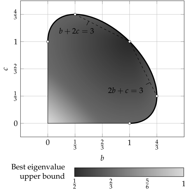
Fig. A.1. A plot of the best possible upper bound on the eigenvalues of (id_3 \otimes \Phi_{b,c}^\dagger)(|v\rangle\langle v|) , which was computed numerically using the semidefinite program (16). This bound agrees with the bounds provided by Lemma A.1 whenever b + c \geq \frac{2}{3} . The area above and to the right of the two dashed lines is covered by the first case of that lemma, whereas the area below and to the left of the dashed lines is covered by the second case of the lemma.
