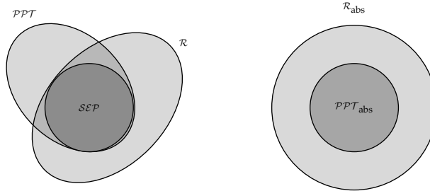
Fig. 1. The figure on the left represents the relationship between the set of separable states \mathcal{SEP} , the set of PPT states \mathcal{PPT} , and the set of states that satisfy the realignment criterion \mathcal{R} . The figure on the right represents the relationship between the set of absolutely PPT states \mathcal{PPT}_{\text{abs}} and the set \mathcal{R}_{\text{abs}} of states that are “absolutely realignable” (see Theorem 1).
